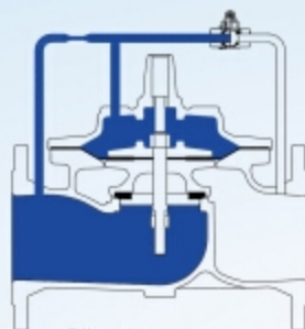
Pilot close Main Valve close
