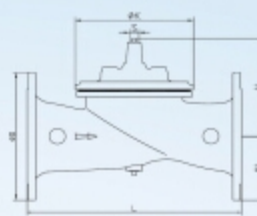
Main Valve-Reduced Bore Type
