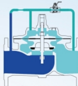
Pilot modulate Main valve modulate
