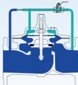
Pilot open Main Valve open
